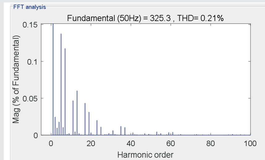
Fig.12. Spectrum of the THD for output voltage
