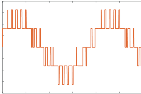
Fig.4. Phase to phase output voltage
