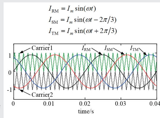
Fig.5.Principle of double-carrier modulation
