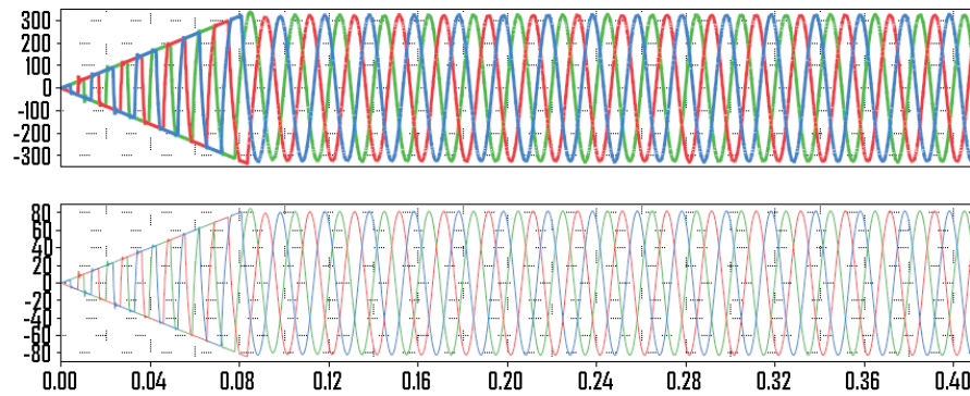
Fig.8. Output voltage (up) and current (down)
