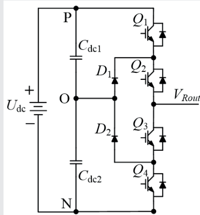
Fig.2. Topology of phase R
